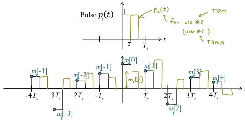
Figure 58: Time sharing in PAM
