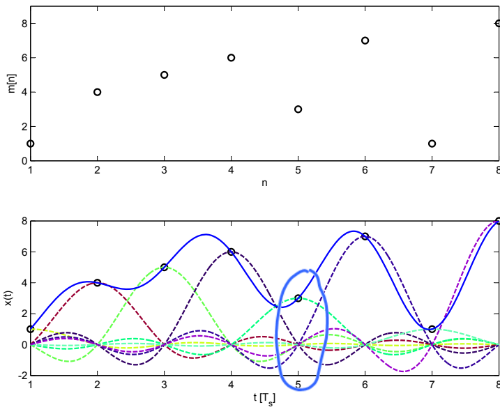
Figure 64: Using the sinc pulse in PAM
