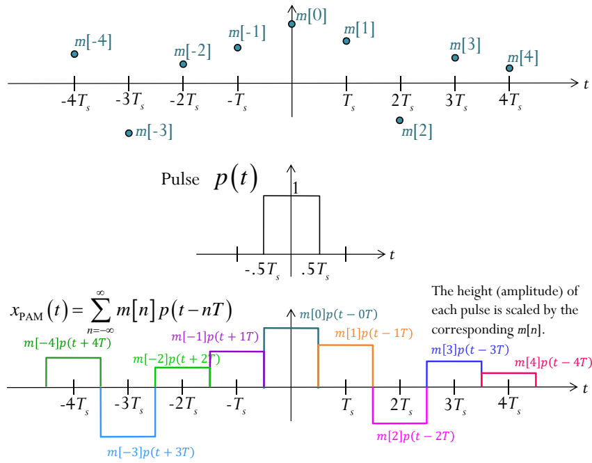
Figure 56: An example of a PAM signal
