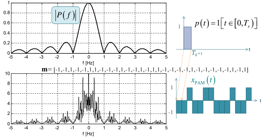
Figure 59: Frequency-Domain Analysis of PAM
