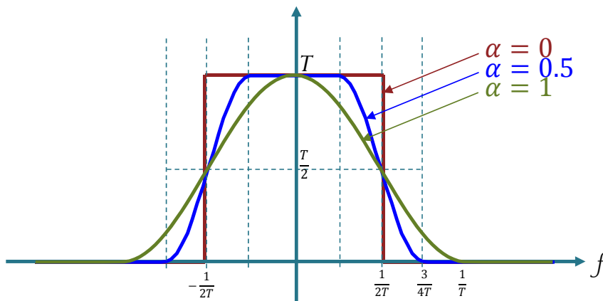
Figure 67: Raised cosine pulse (in the frequency domain) with different values of the roll-off factor
