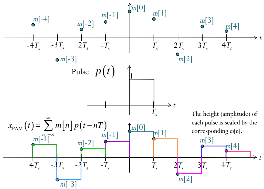
Figure 57: Another Example of a PAM signal
