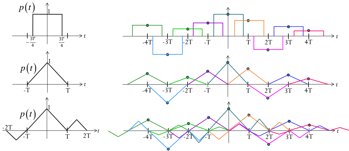
Figure 63: Examples of pulses that do not cause ISI.
