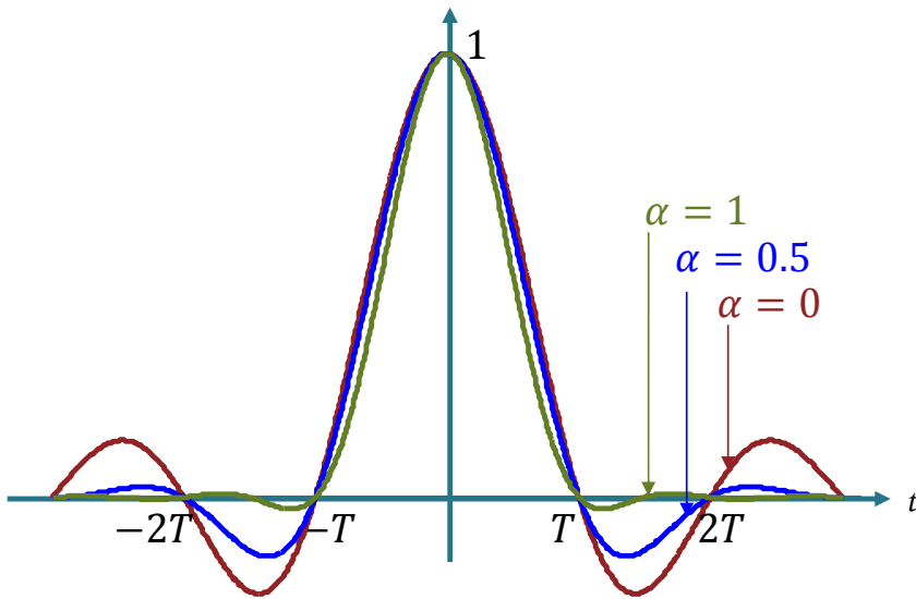
Figure 68: Raised cosine pulse (in the time domain) with different values of the roll-off factor
