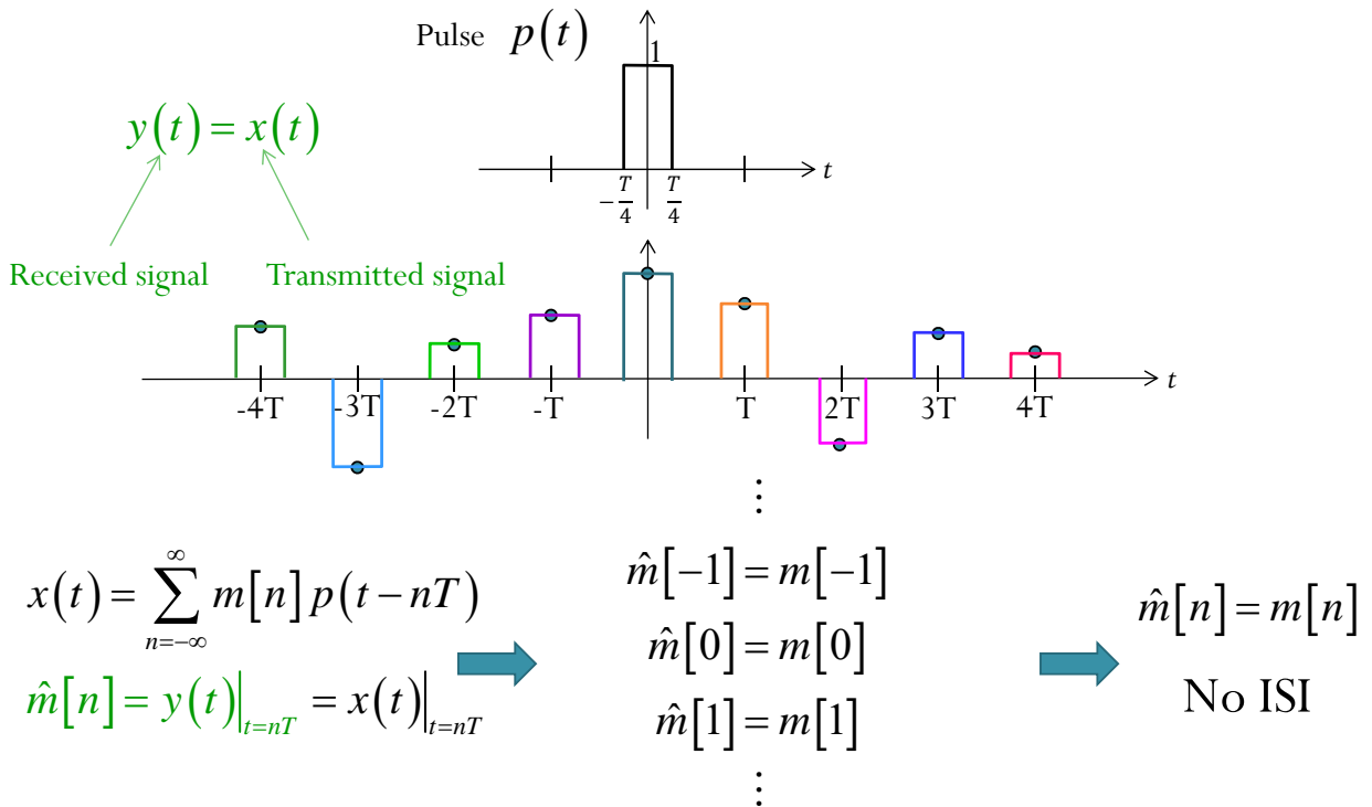
Figure 62: PAM using narrow pulses
