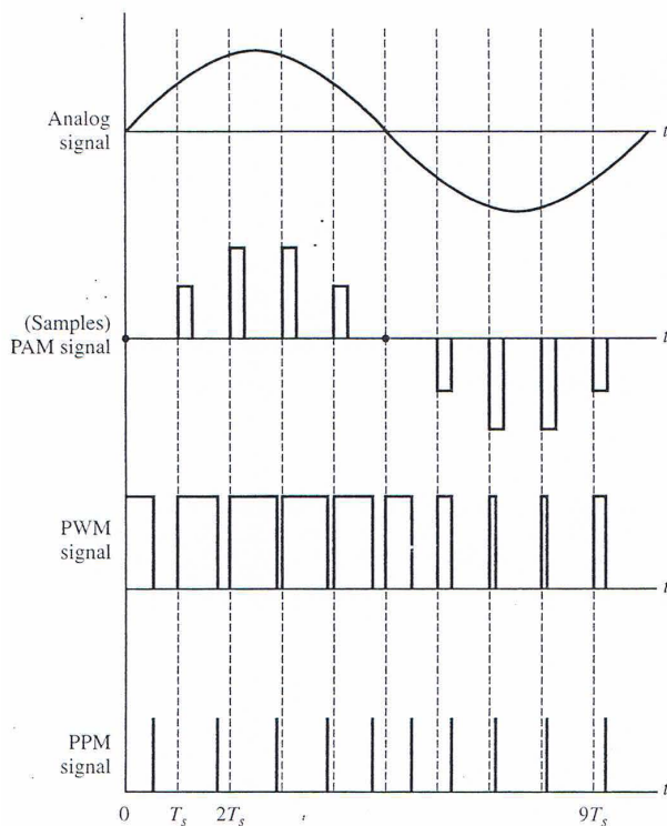
Figure 55: Illustration of PAM, PWM, and PPM. [14, Fig. 3.56]
