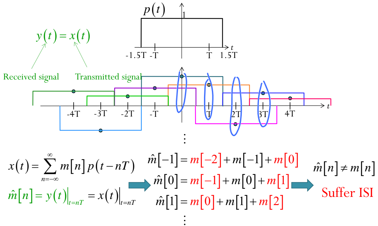
Figure 61: ISI in PAM
