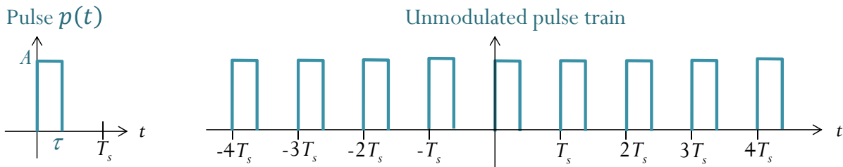
Figure 54: Unmodulated pulse train
